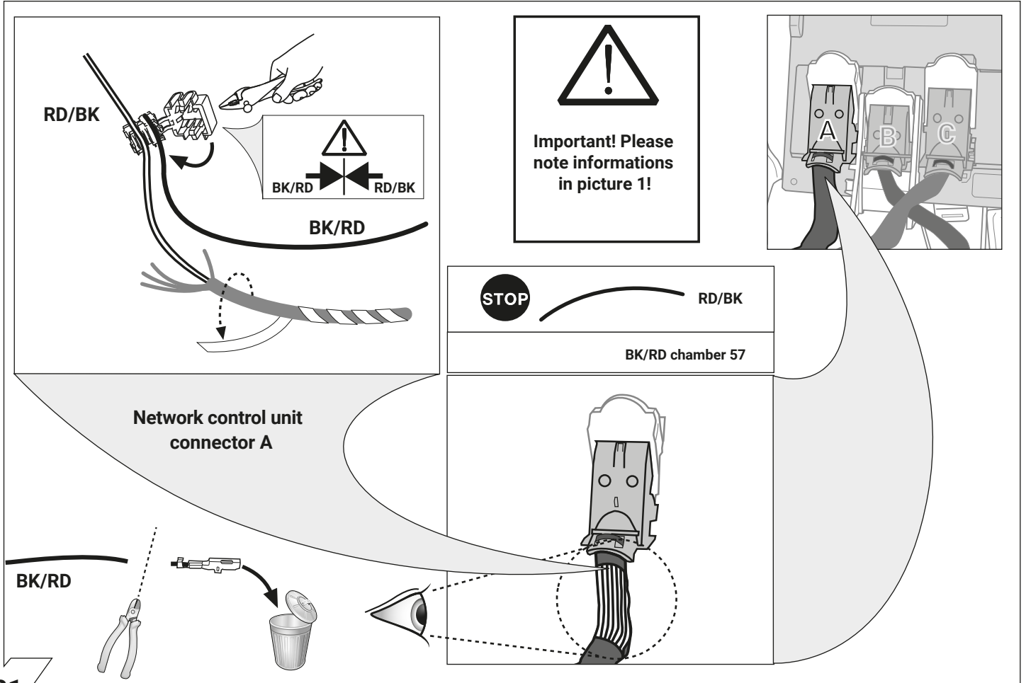
CAN-Data Wire
